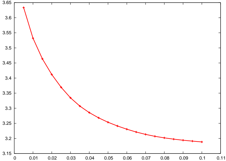
Figure 8: AVaR as a function of nominal suboptimality
